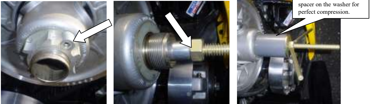
QRS Helix Removal Tool (151-106)
